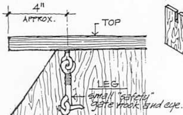
Fastening Top to Legs Detail
